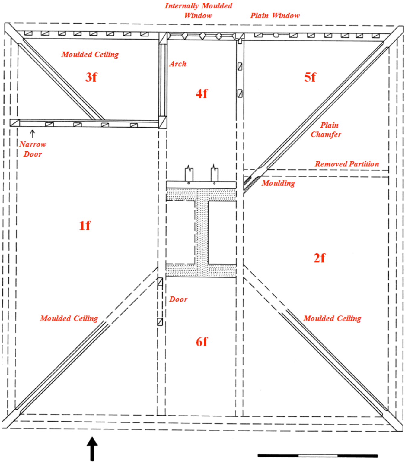
Letheringham Lodge Reconstruction of Original First Floor Plan
